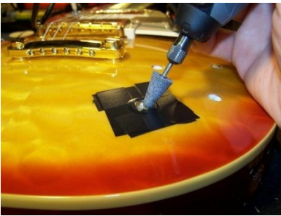
Fig. 3 Widen the top of the hole
